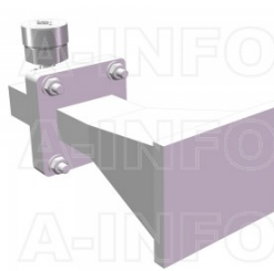
LB-112-10-C-7SPO Standard Gain Horn Antenna 7.05-10GHz 10dB Gain 7mm Female
